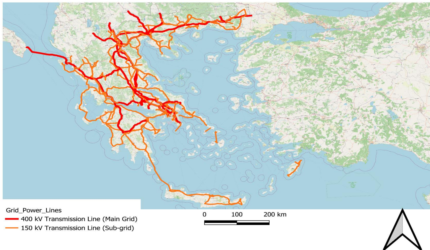
Map 2: High-Voltage Transmission Grid
