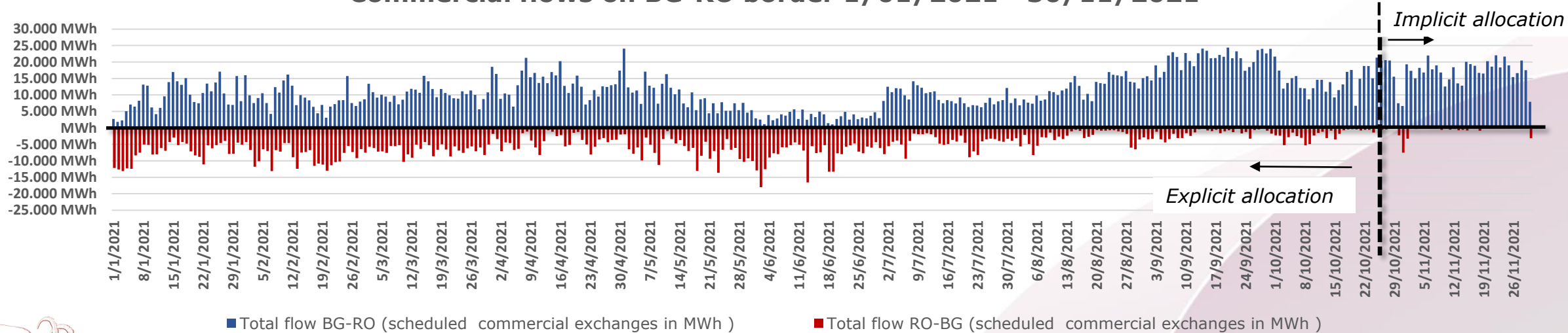
Commercial flows on BG-RO border 1/01/2021 - 30/11/2021
