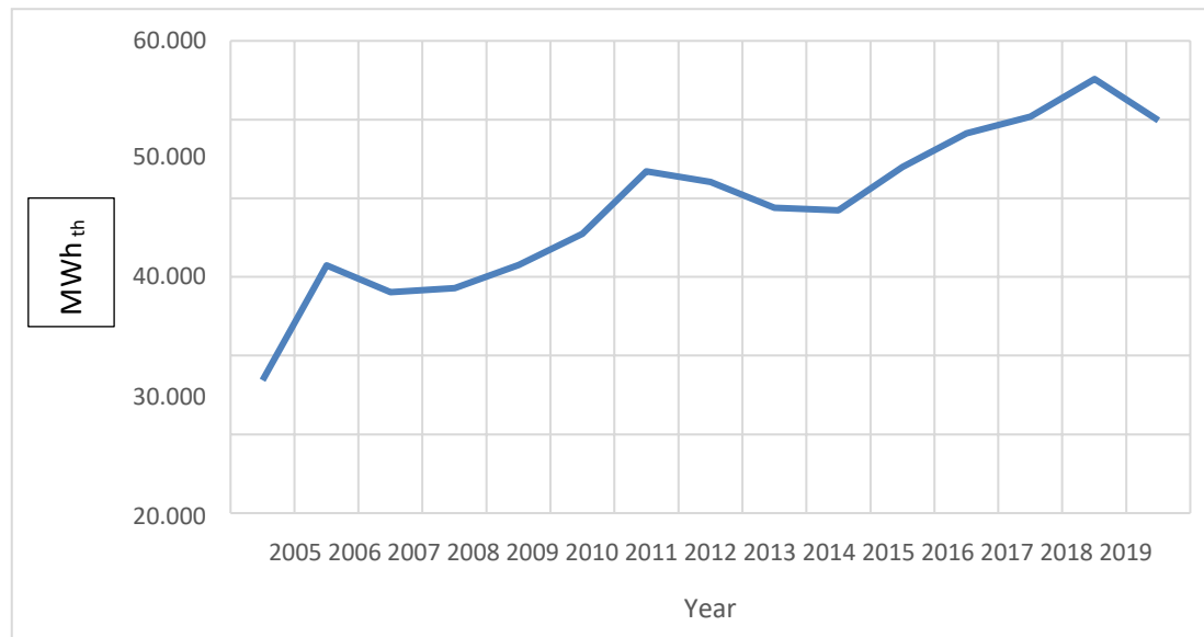
Diagram 17 - Annual Thermal Energy Supply from the Units of the Amyntaio TPP into the DHS of the City of Amyntaio, 2005-2019
