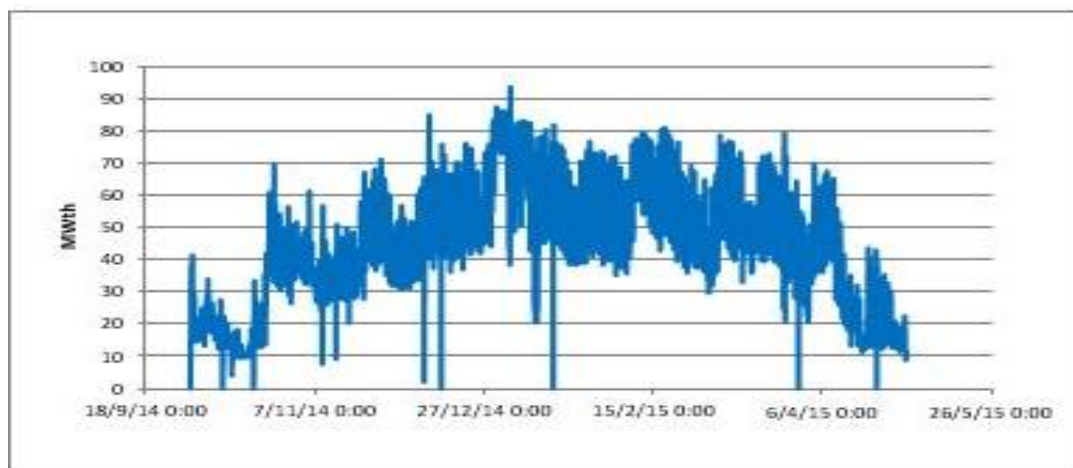
Diagram 13 - Distribution of Total Hourly Thermal Energy Demand of DHS of Ptolemaida, 2014-2015
