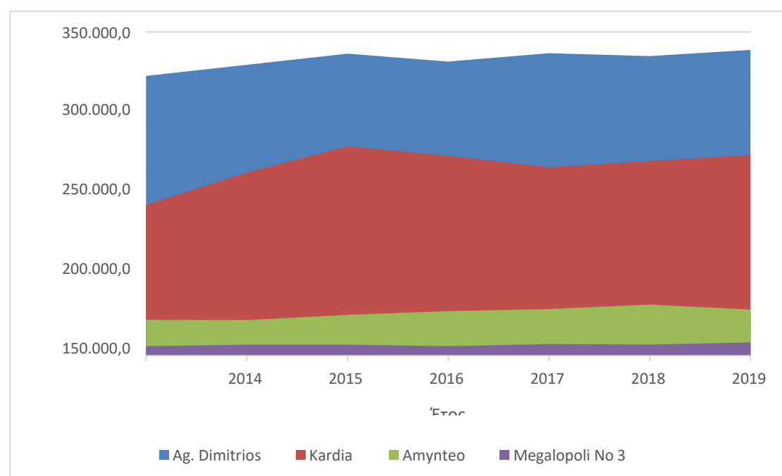
Diagram 19 - Annual Thermal Consumption, in MWh th , of All DHS Operating with Lignite Power Plants, 2013-2019
